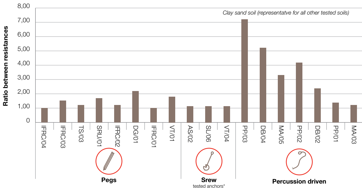
Ratios between the maximum resistance measured without and with a 5 cm displacement constraint
