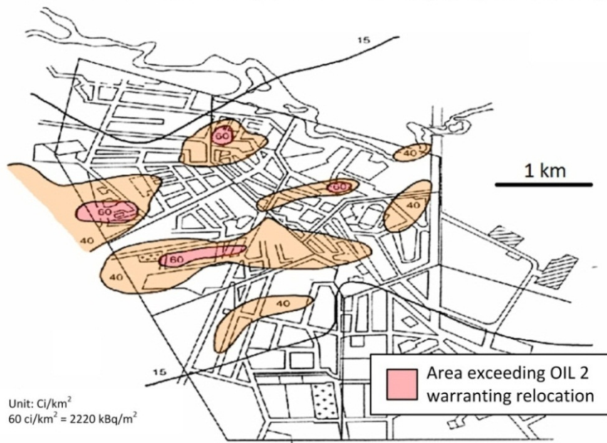
Cesium-137 and cesium-134 deposition in Polesskoe (50 km from Chernobyl)
