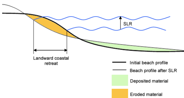
Figure 1: Model of landward coastal retreat under Sea Level Rise (SLR)
